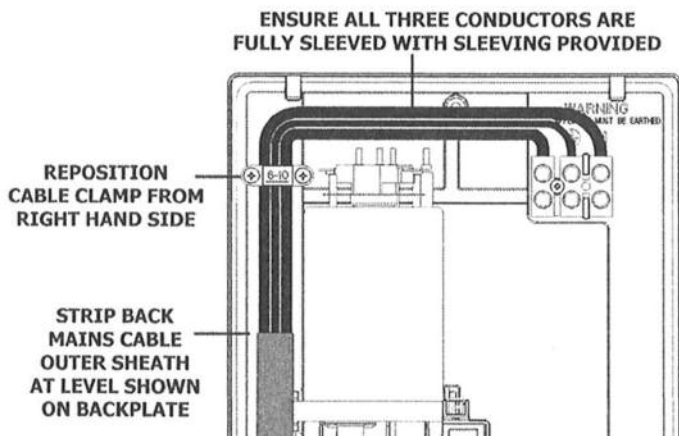
Diagram 3a Left Side Installation
